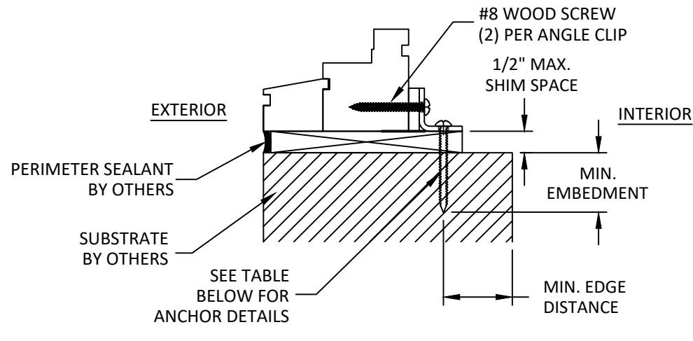
D 5 VERTICAL SECTION SILL - ANGLE CLIP
