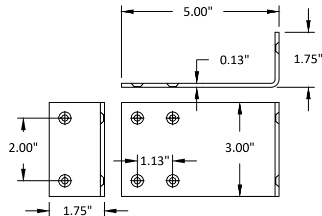
15 ANGLE CLIP 304 STAINLESS STEEL
