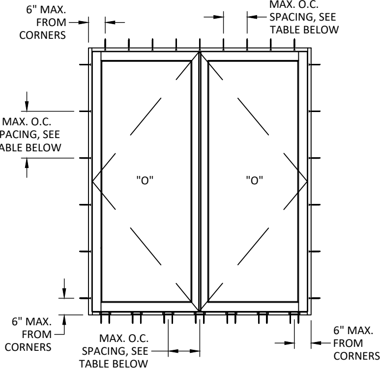
ANCHOR LAYOUT THROUGH FRAME - HEAD & JAMBS ANGLE CLIP - SILL
