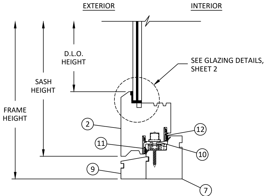
B 6 VERTICAL SECTION SILL
