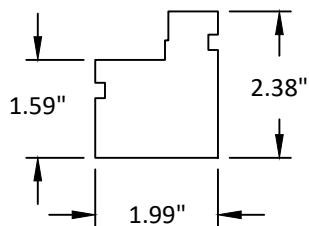
7 SILL MAHOGANY
