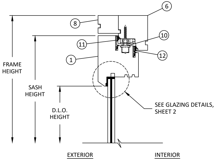
A 6 VERTICAL SECTION HEAD
