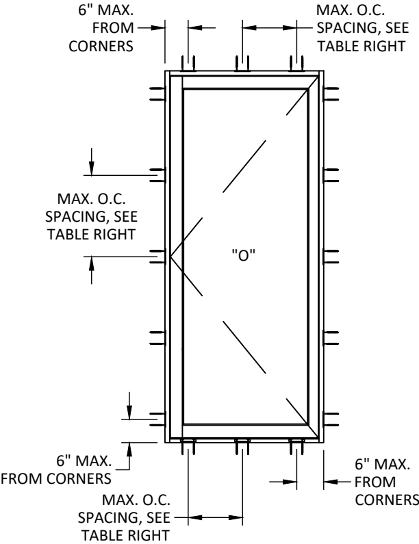
ANCHOR LAYOUT FLAT CLIP - HEAD & JAMBS ANGLE CLIP - SILL
