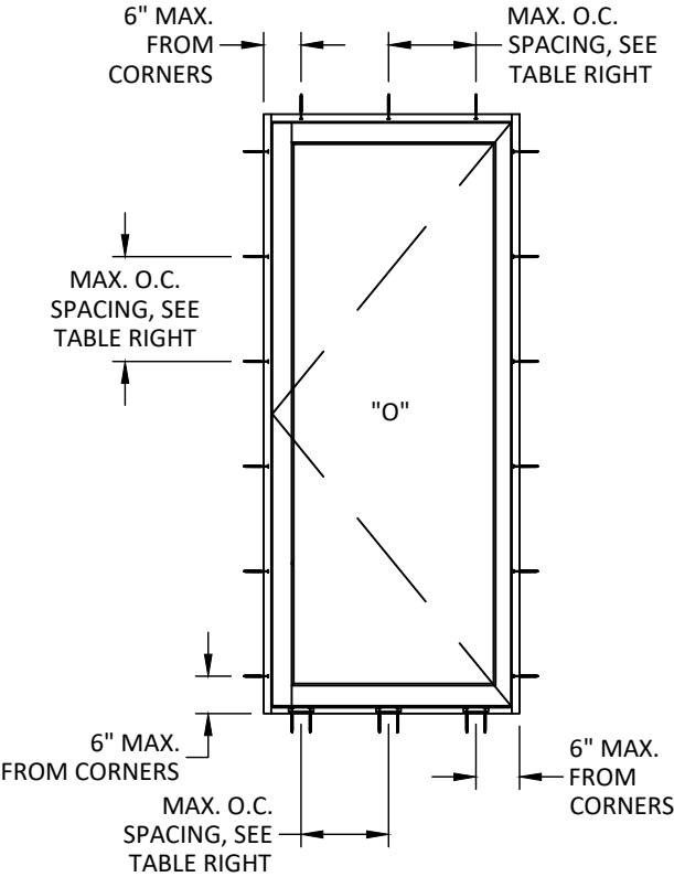
ANCHOR LAYOUT THROUGH FRAME - HEAD & JAMBS ANGLE CLIP - SILL
